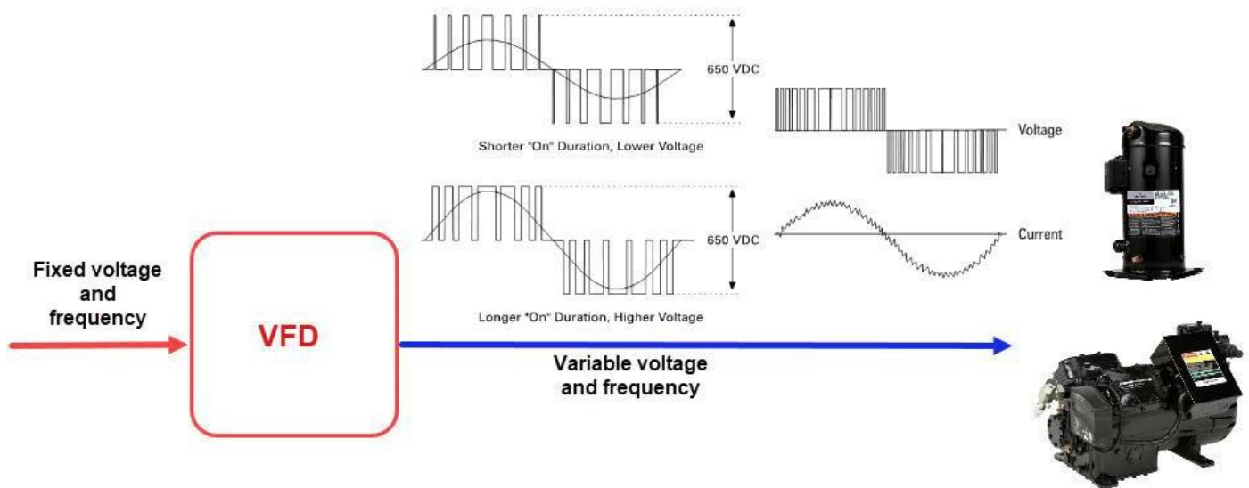
Figure 2 – Utility vs VFD voltage waveform
